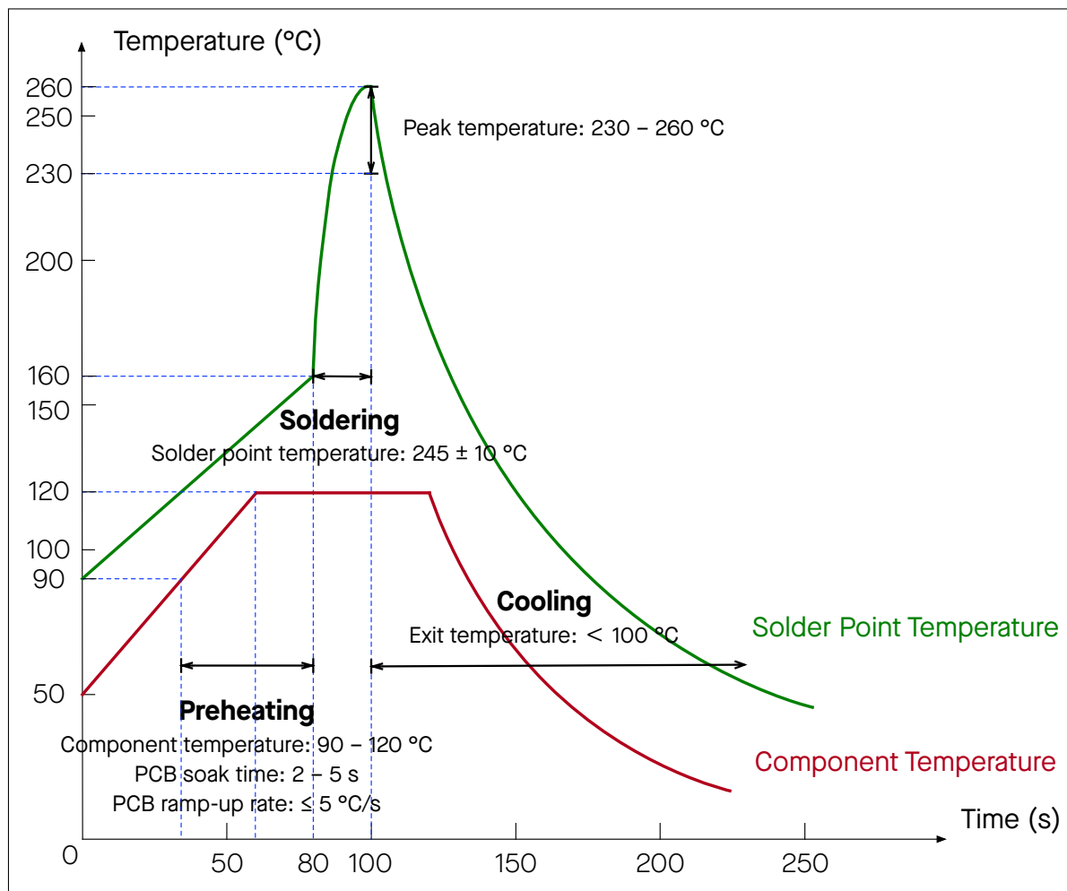
Figure 10: Wave Soldering Profile
