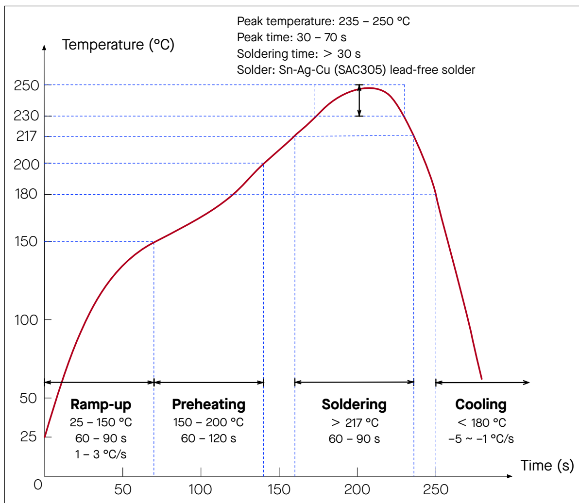
Figure 9: Reflow Profile
